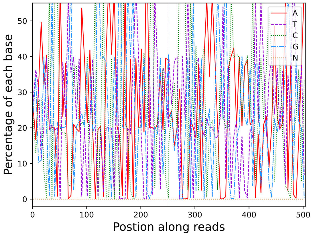
Base percentage along reads (R10821)
